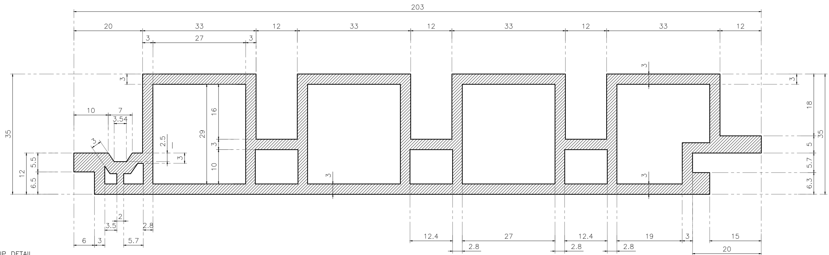
BLOW UP DETAIL WPO18035 SCALE 1.5:1 MTS
